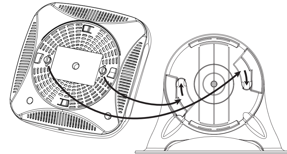
Figure 3 Stand Installation
